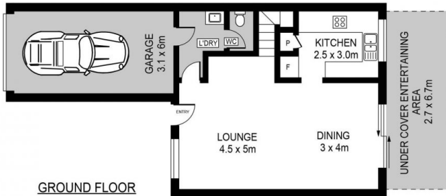
GROUND FLOOR
